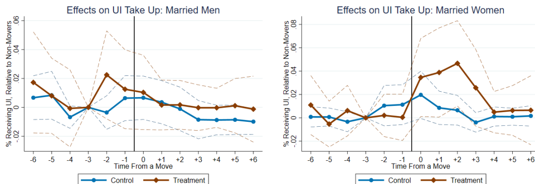
Figure 3: Effects of UI Eligibility on UI Take-Up for Men (left) and Women (right)
